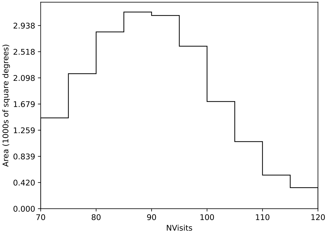
too_elab_r256_d2_ugrizy_v3.4_10yrs Yr 1 all bands: NVisits
