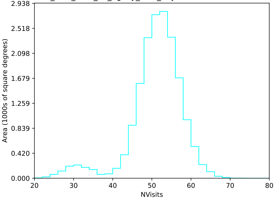
too_elab_r256_d2_ugrizy_v3.4_10yrs WFD u band: NVisits
