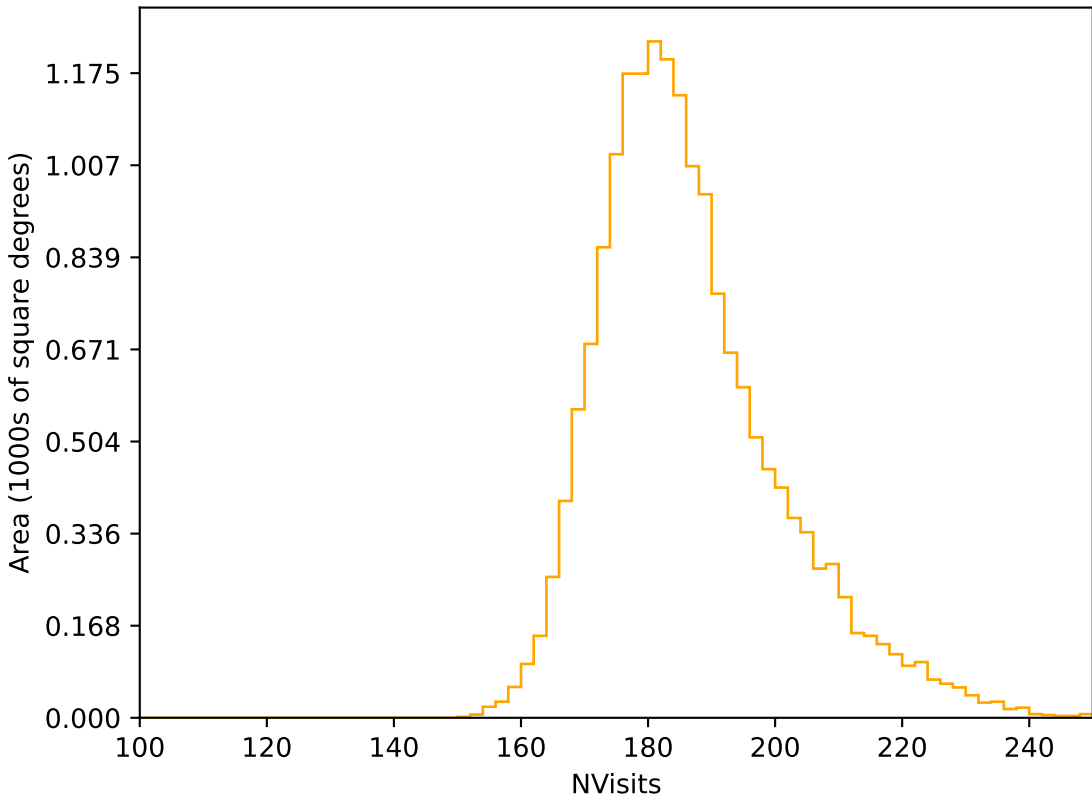
too_elab_r256_d2_ugrizy_v3.4_10yrs WFD r band: NVisits
