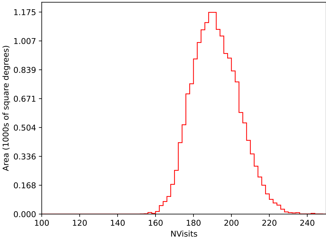
too_elab_r256_d2_ugrizy_v3.4_10yrs WFD i band: NVisits
