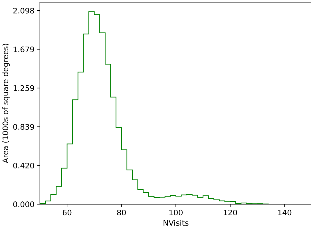
too_elab_r256_d2_ugrizy_v3.4_10yrs WFD g band: NVisits
