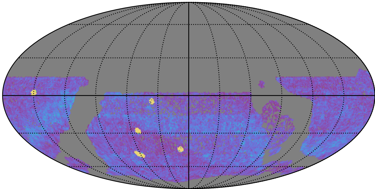
too_elab_r256_d2_ugrizy_v3.4_10yrs WFD all bands: NVisits
