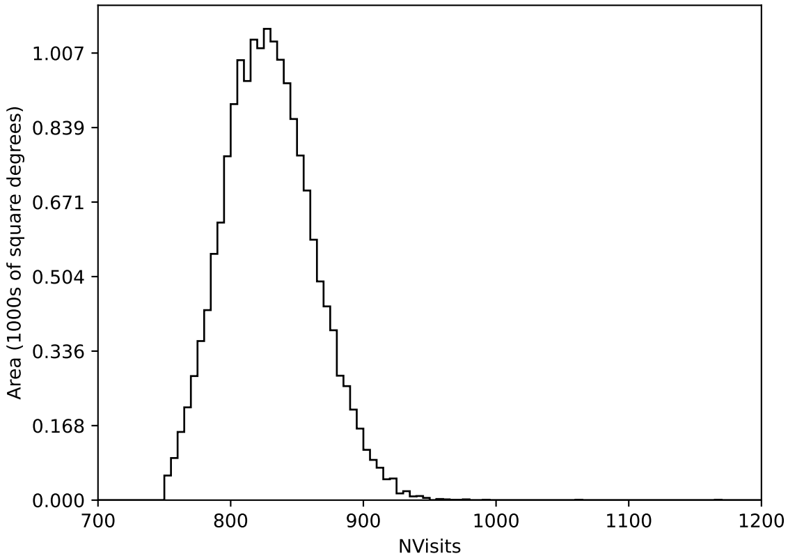
too_elab_r256_d2_ugrizy_v3.4_10yrs WFD all bands: NVisits
