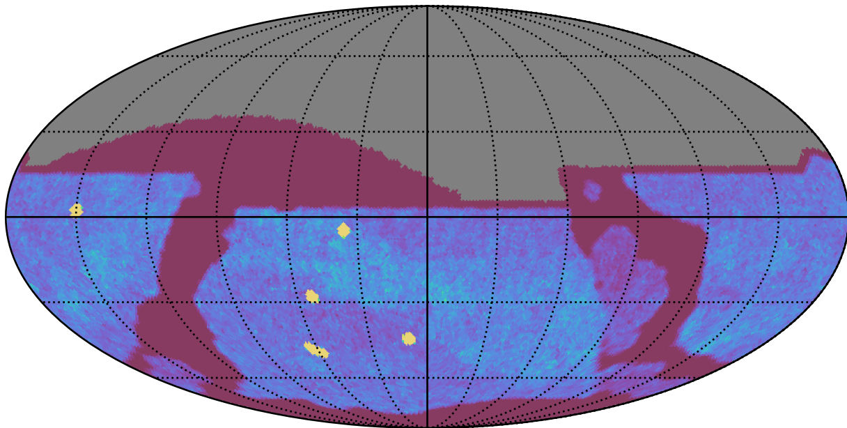
too_elab_r256_d2_ugrizy_v3.4_10yrs All sky z band: NVisits
