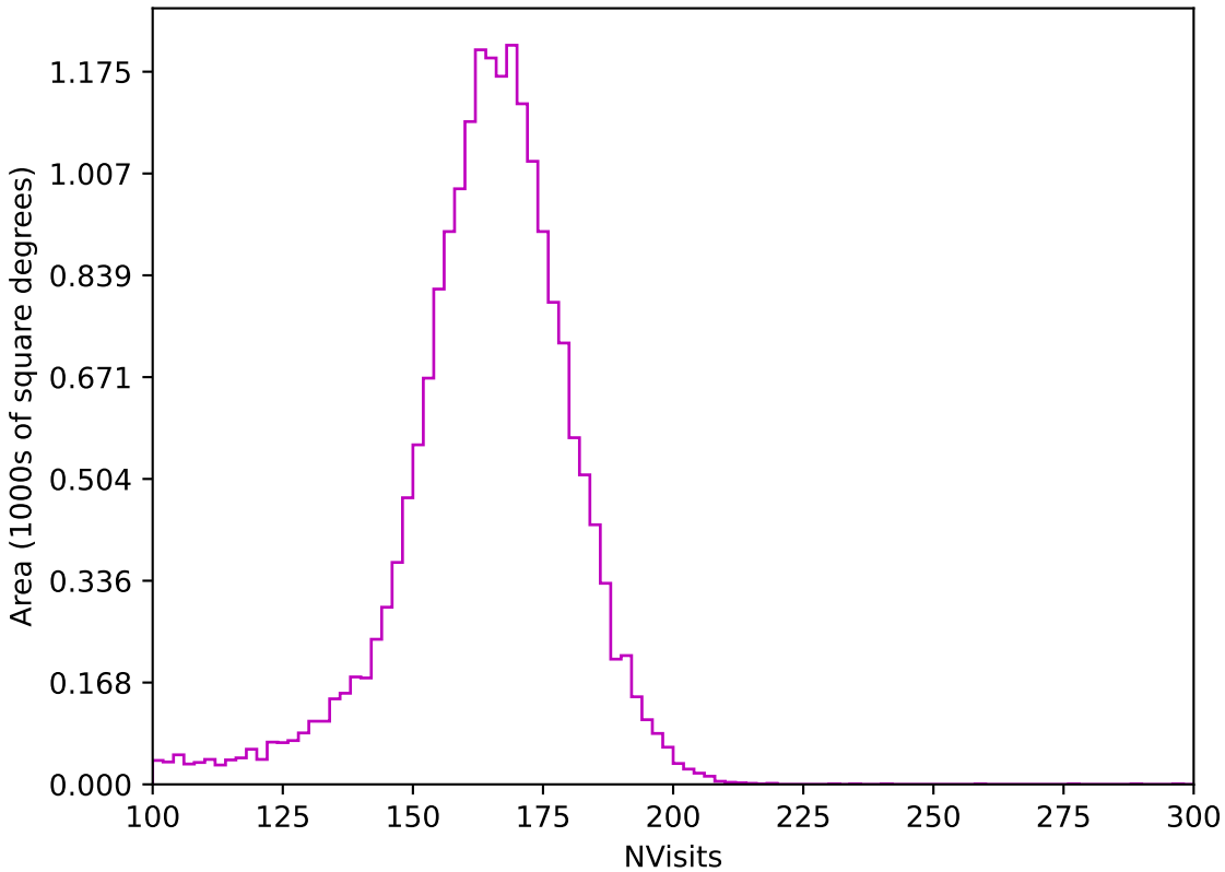
too_elab_r256_d2_ugrizy_v3.4_10yrs All sky z band: NVisits
