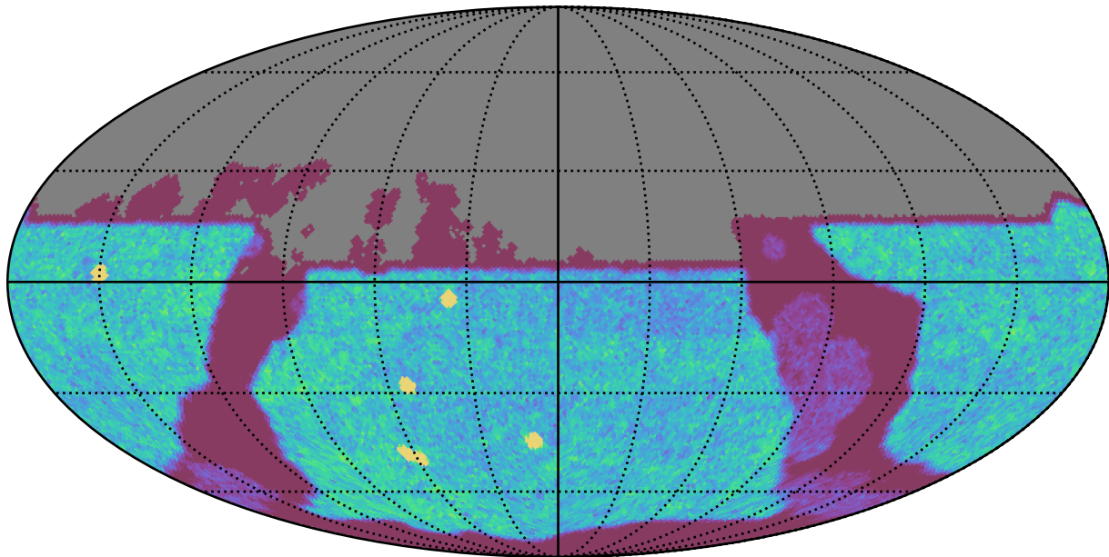
too_elab_r256_d2_ugrizy_v3.4_10yrs All sky u band: NVisits
