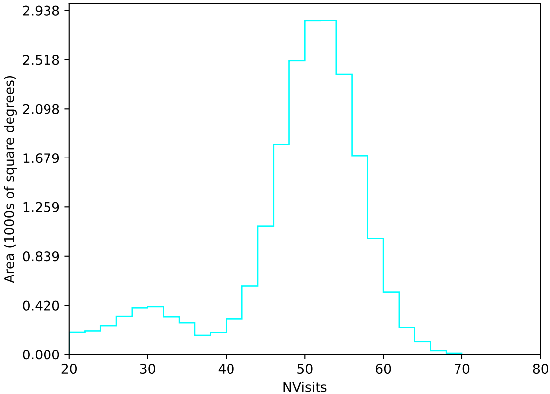
too_elab_r256_d2_ugrizy_v3.4_10yrs All sky u band: NVisits
