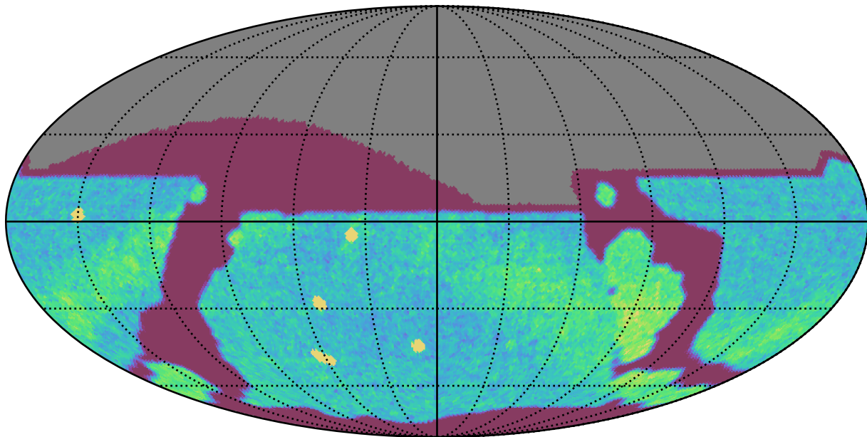
too_elab_r256_d2_ugrizy_v3.4_10yrs All sky r band: NVisits
