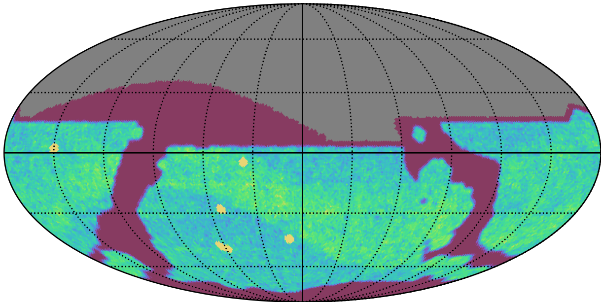
too_elab_r256_d2_ugrizy_v3.4_10yrs All sky i band: NVisits
