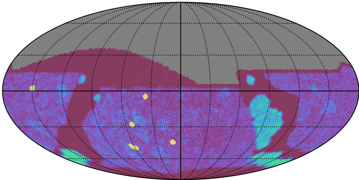
too_elab_r256_d2_ugrizy_v3.4_10yrs All sky g band: NVisits
