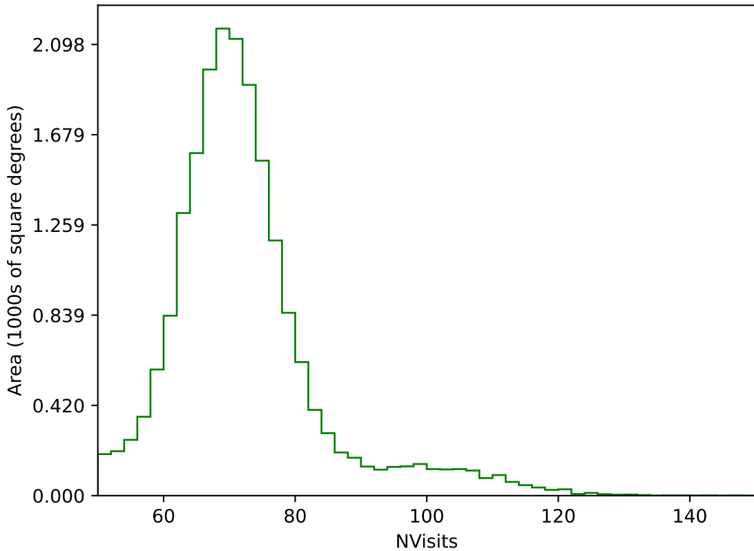
too_elab_r256_d2_ugrizy_v3.4_10yrs All sky g band: NVisits
