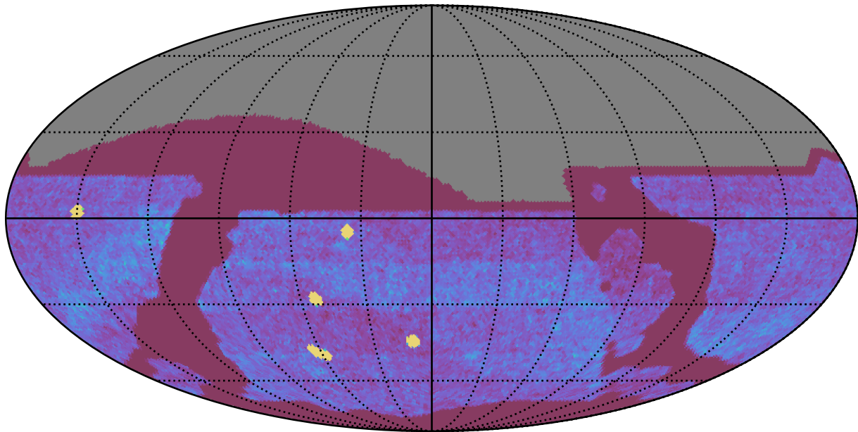
too_elab_r256_d2_ugrizy_v3.4_10yrs All sky all bands: NVisits
