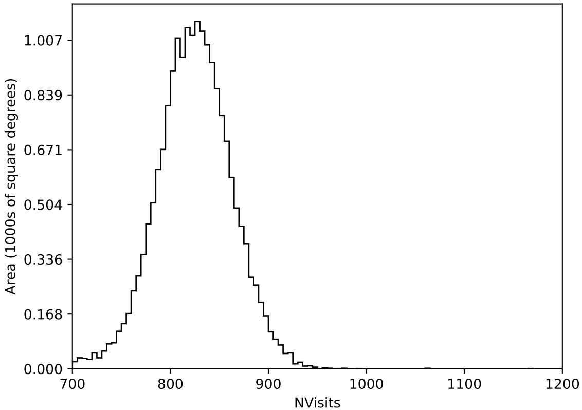
too_elab_r256_d2_ugrizy_v3.4_10yrs All sky all bands: NVisits
