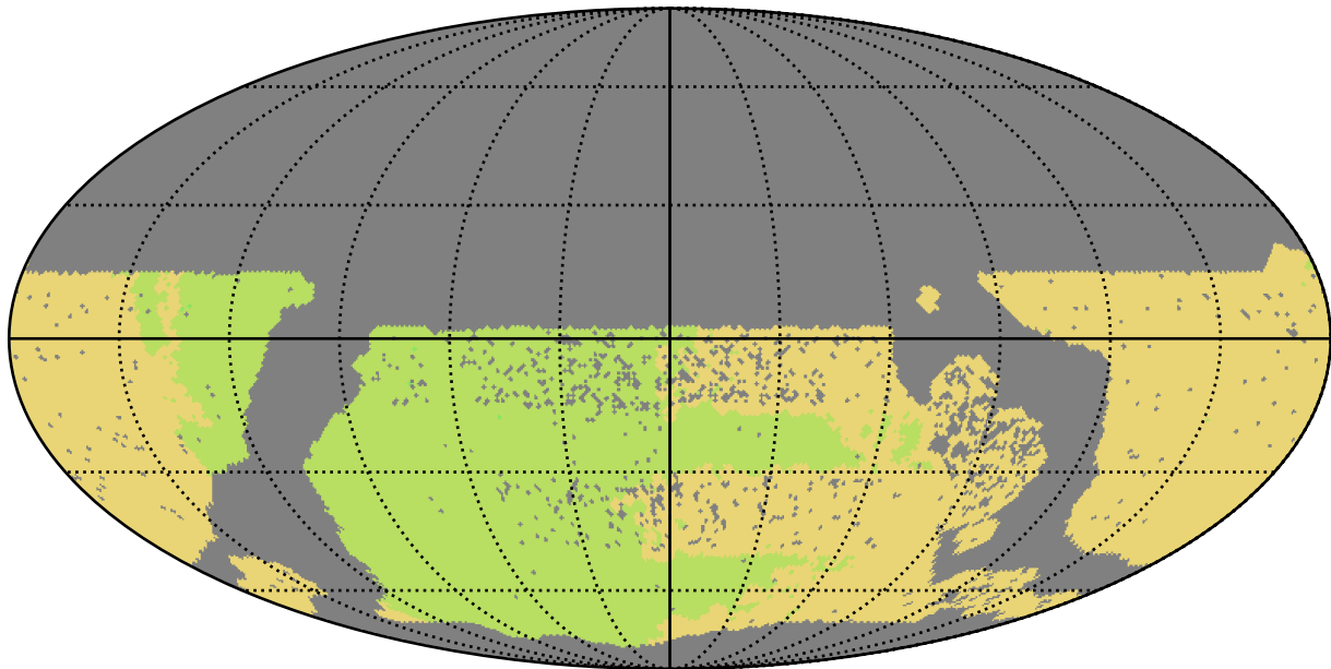
too_elab_r256_d2_ugrizy_v3.4_10yrs WFD all bands: NSeasons
