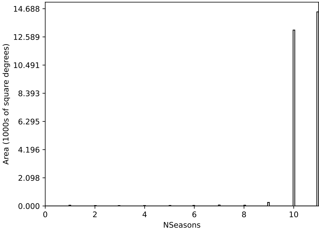
too_elab_r256_d2_ugrizy_v3.4_10yrs All sky all bands: NSeasons
