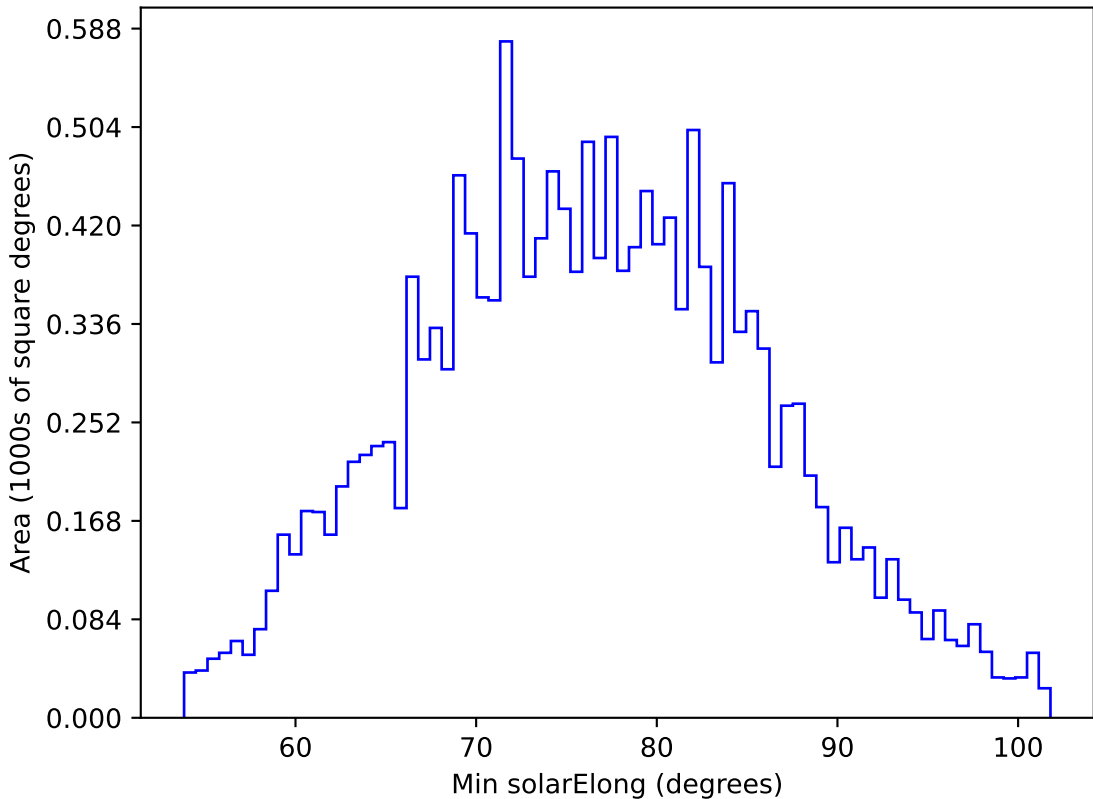
too_elab_r256_d2_ugrizy_v3.4_10yrs WFD u band: Min solarElong
