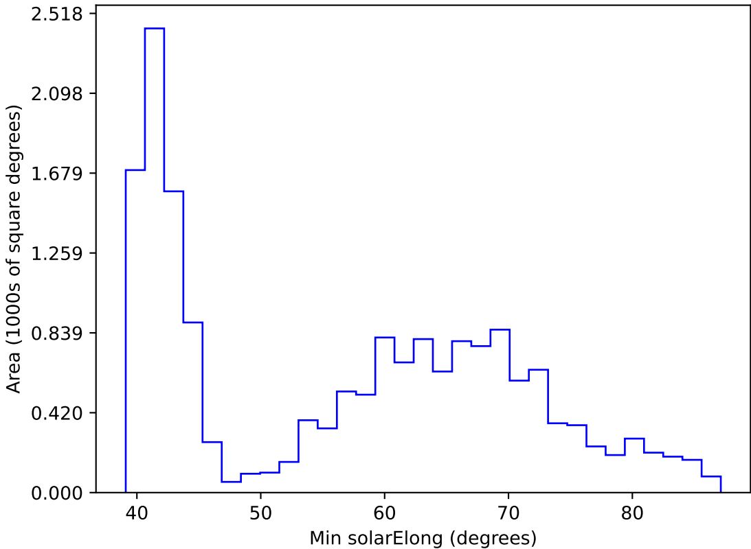
too_elab_r256_d2_ugrizy_v3.4_10yrs WFD r band: Min solarElong
