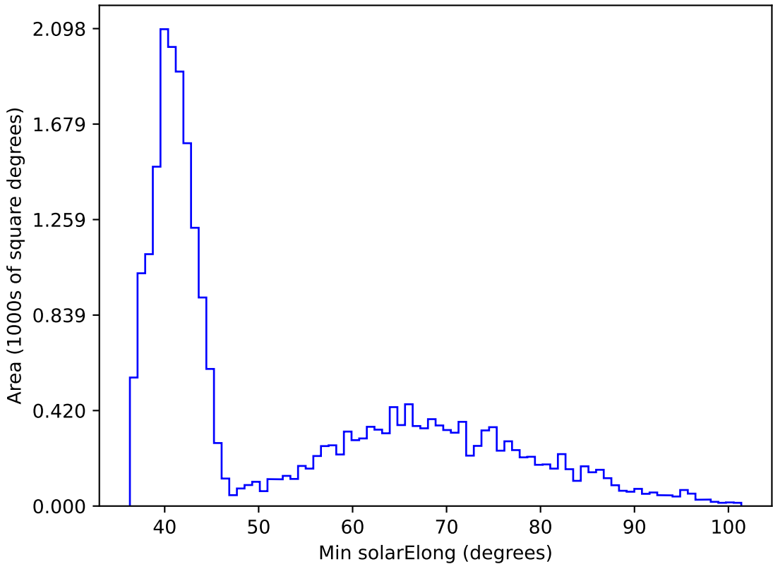
too_elab_r256_d2_ugrizy_v3.4_10yrs All sky z band: Min solarElong
