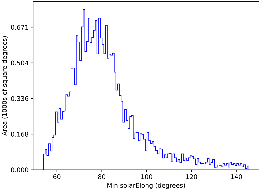
too_elab_r256_d2_ugrizy_v3.4_10yrs All sky u band: Min solarElong
