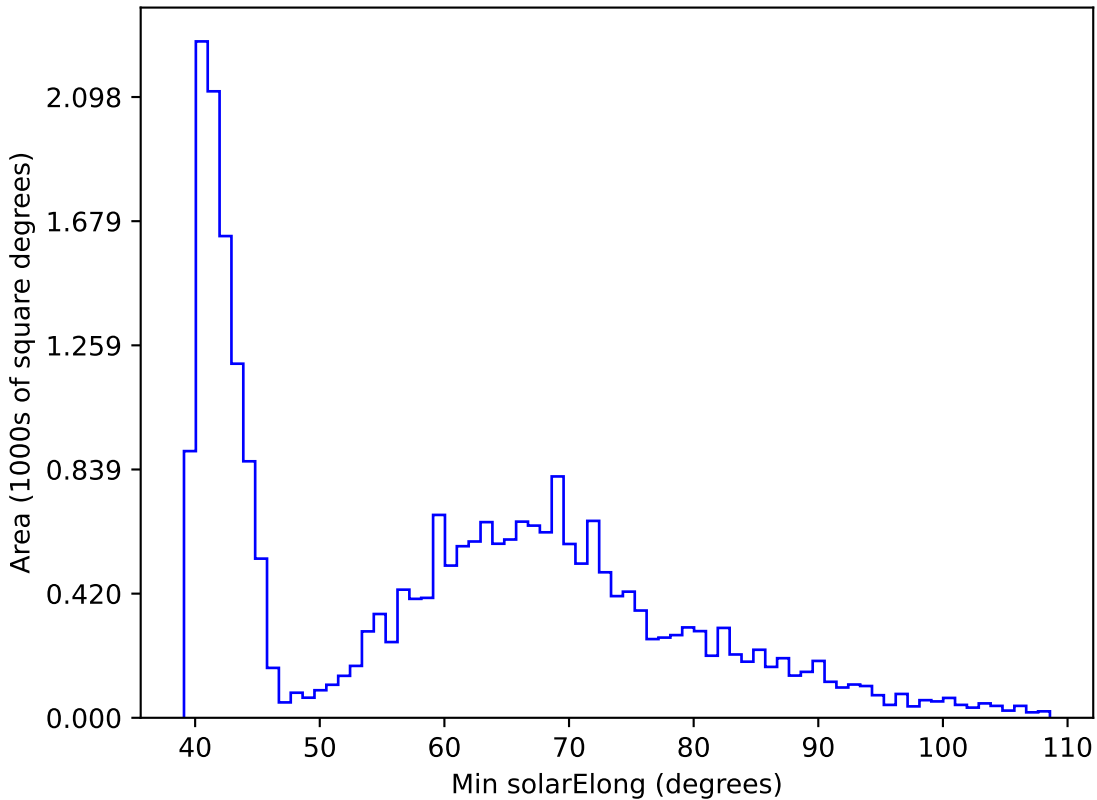
too_elab_r256_d2_ugrizy_v3.4_10yrs All sky r band: Min solarElong
