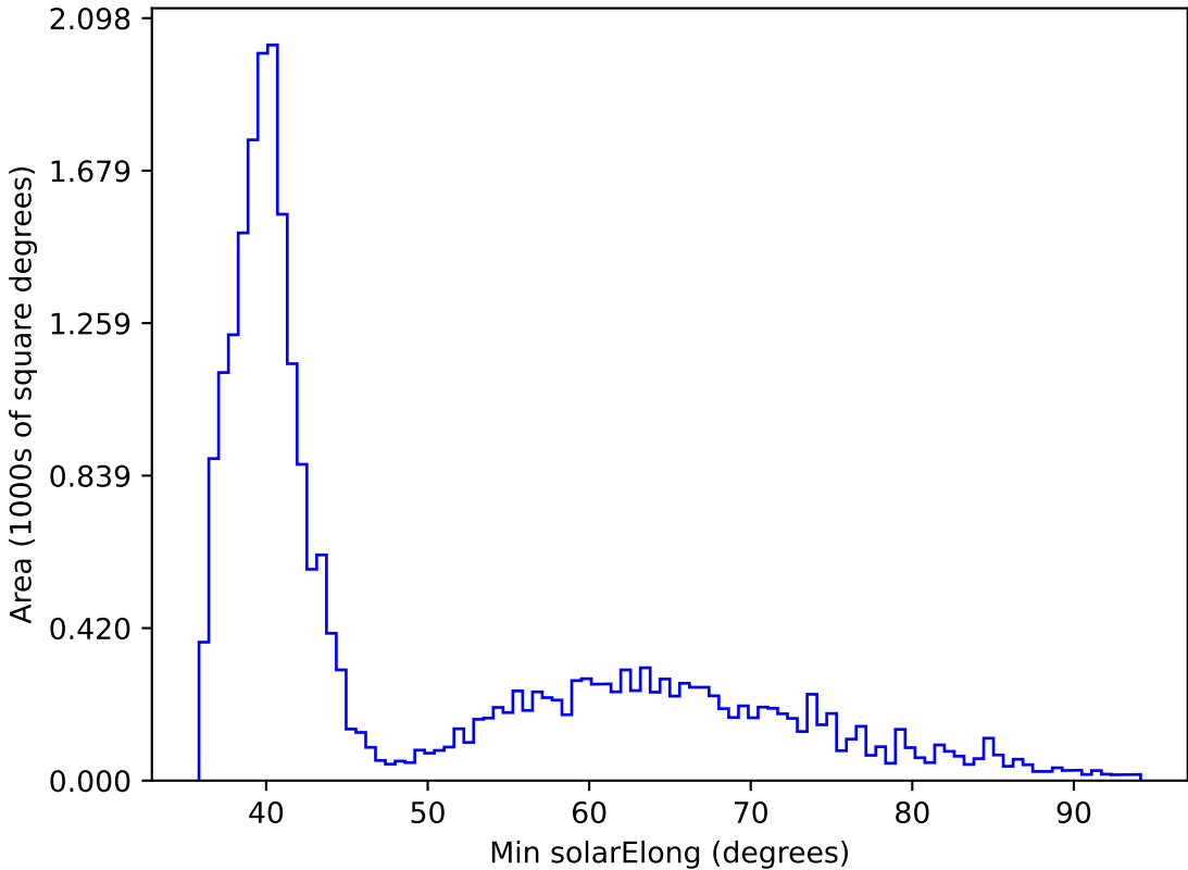
too_elab_r256_d2_ugrizy_v3.4_10yrs All sky all bands: Min solarElong
