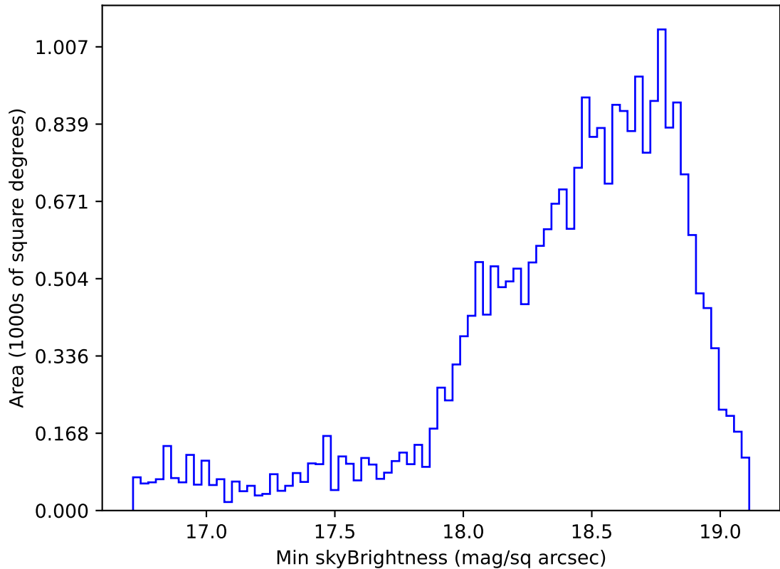
too_elab_r256_d2_ugrizy_v3.4_10yrs Yr 1 z band: Min skyBrightness
