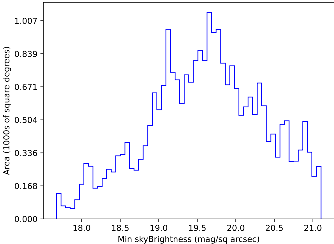
too_elab_r256_d2_ugrizy_v3.4_10yrs Yr 1 r band: Min skyBrightness
