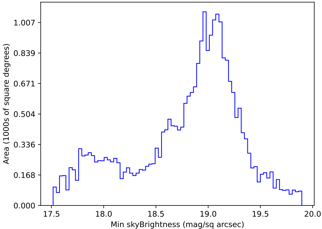
too_elab_r256_d2_ugrizy_v3.4_10yrs Yr 1 i band: Min skyBrightness
