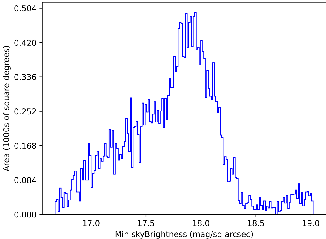
too_elab_r256_d2_ugrizy_v3.4_10yrs Yr 1 all bands: Min skyBrightness
