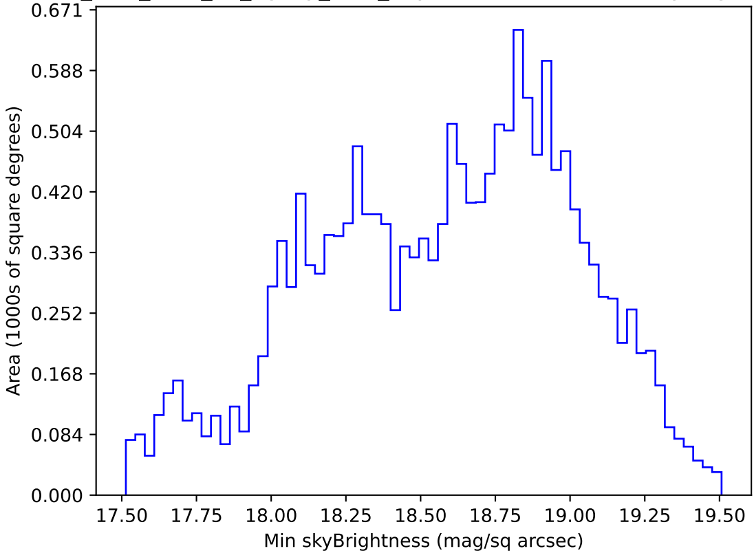
too_elab_r256_d2_ugrizy_v3.4_10yrs WFD r band: Min skyBrightness
