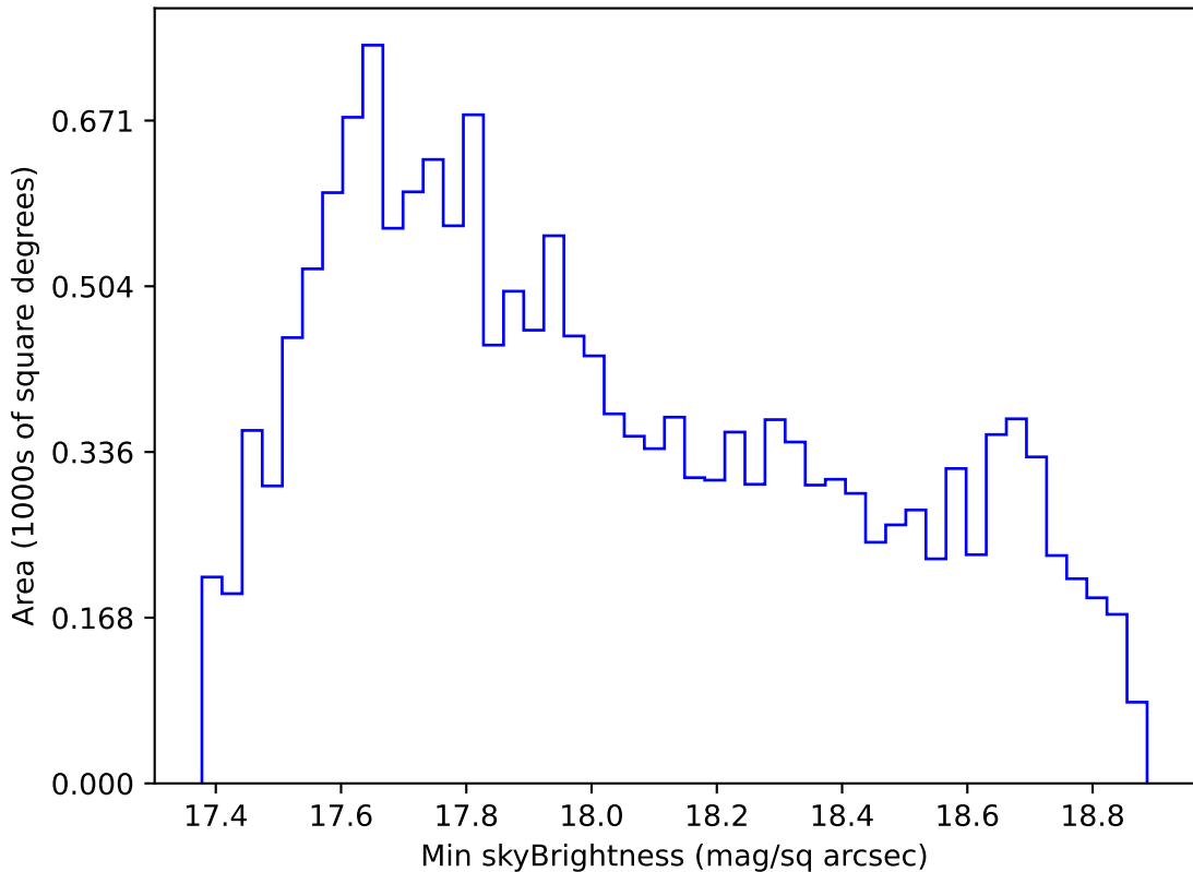
too_elab_r256_d2_ugrizy_v3.4_10yrs WFD i band: Min skyBrightness
