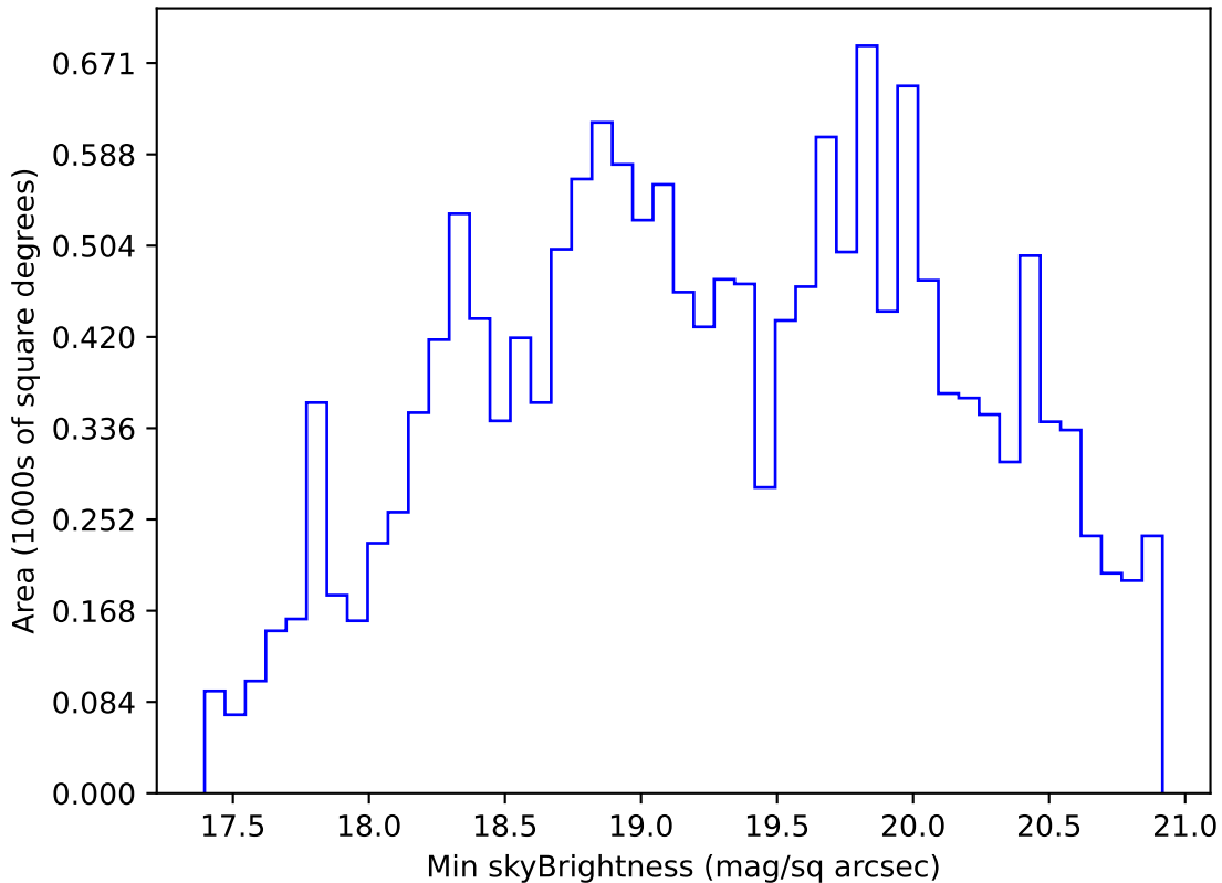
too_elab_r256_d2_ugrizy_v3.4_10yrs WFD g band: Min skyBrightness
