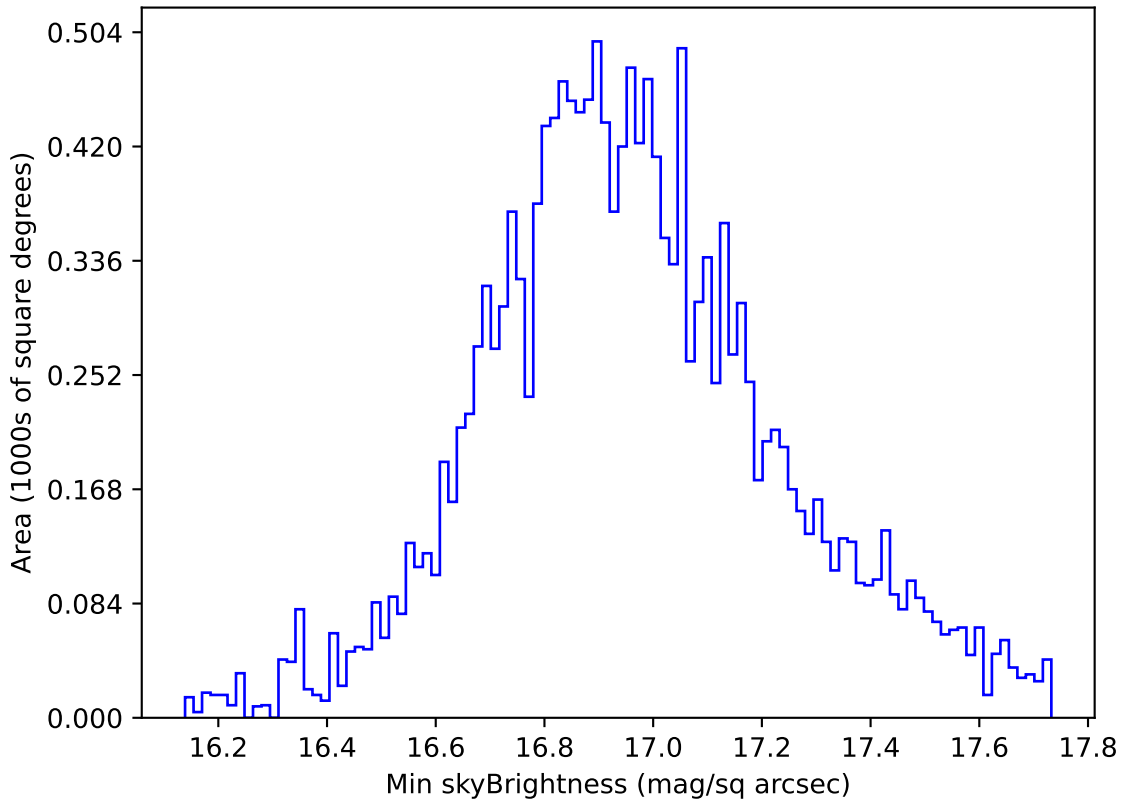
too_elab_r256_d2_ugrizy_v3.4_10yrs WFD all bands: Min skyBrightness
