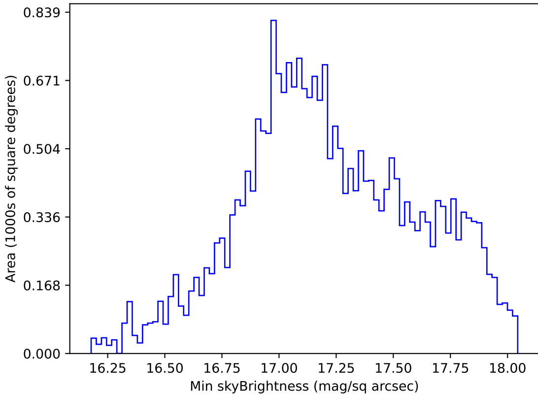
too_elab_r256_d2_ugrizy_v3.4_10yrs All sky y band: Min skyBrightness
