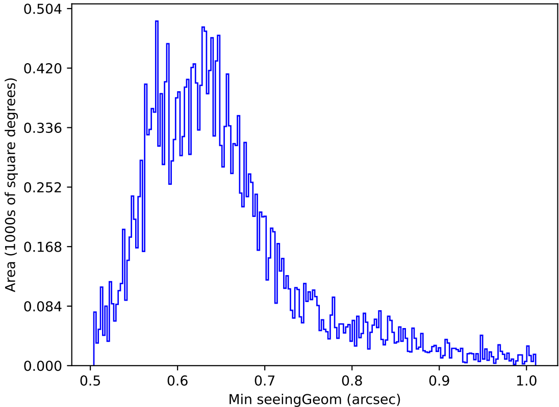
too_elab_r256_d2_ugrizy_v3.4_10yrs Yr 1 z band: Min seeingGeom
