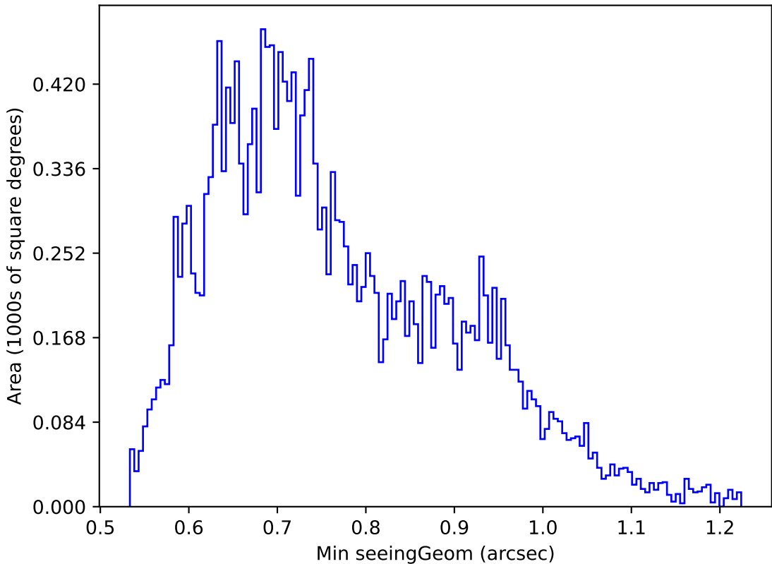
too_elab_r256_d2_ugrizy_v3.4_10yrs Yr 1 u band: Min seeingGeom
