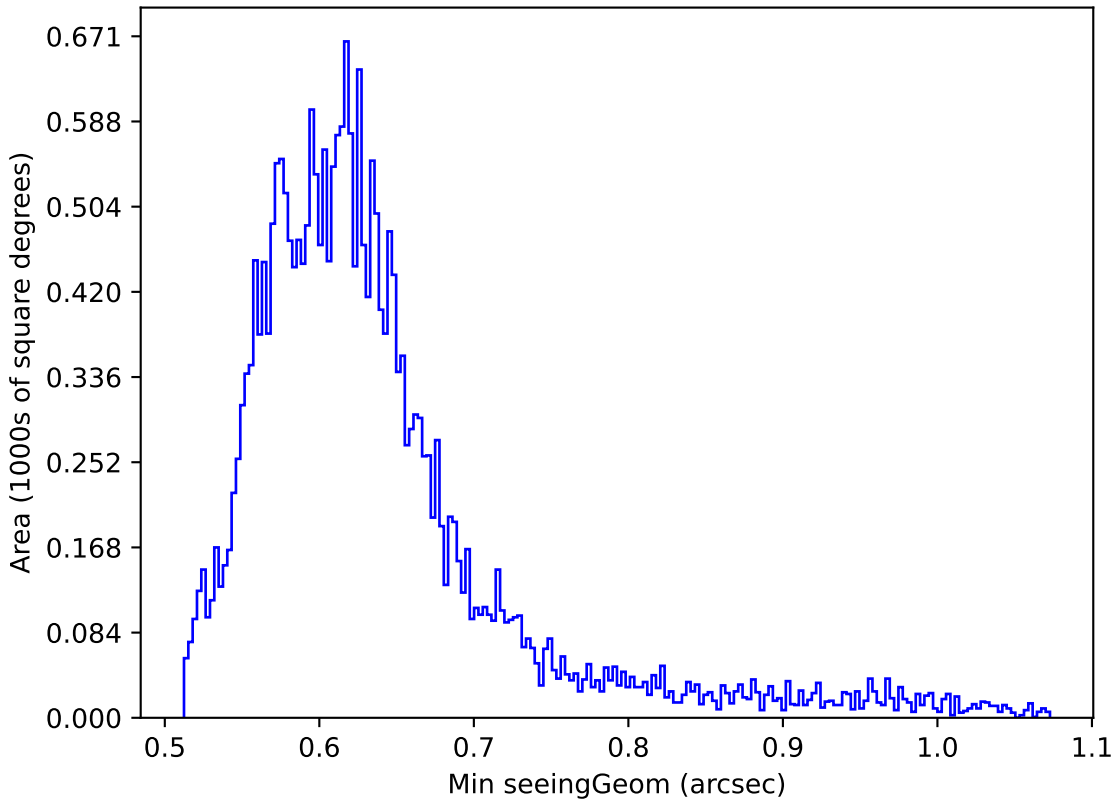
too_elab_r256_d2_ugrizy_v3.4_10yrs Yr 1 r band: Min seeingGeom
