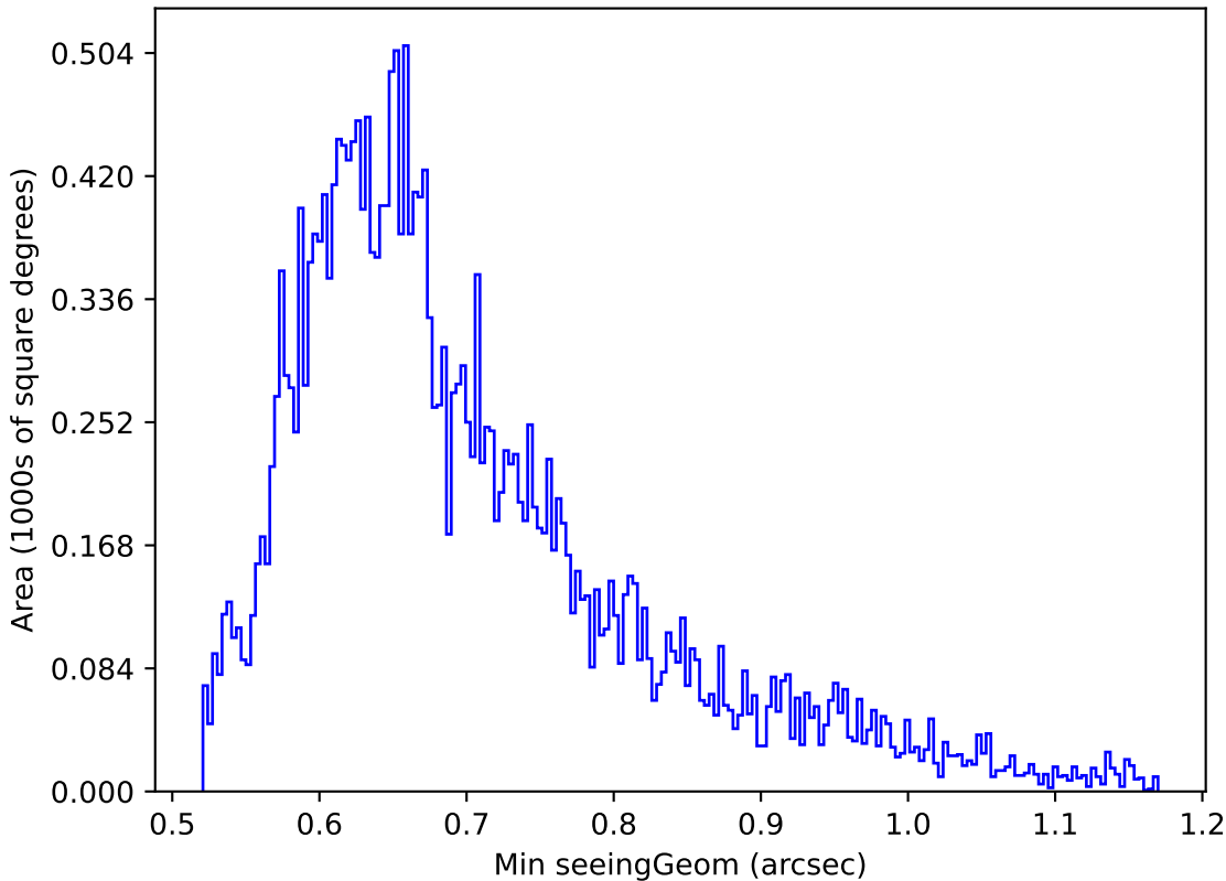
too_elab_r256_d2_ugrizy_v3.4_10yrs Yr 1 g band: Min seeingGeom
