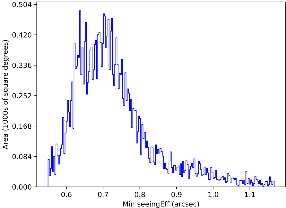
too_elab_r256_d2_ugrizy_v3.4_10yrs Yr 1 z band: Min seeingEff
