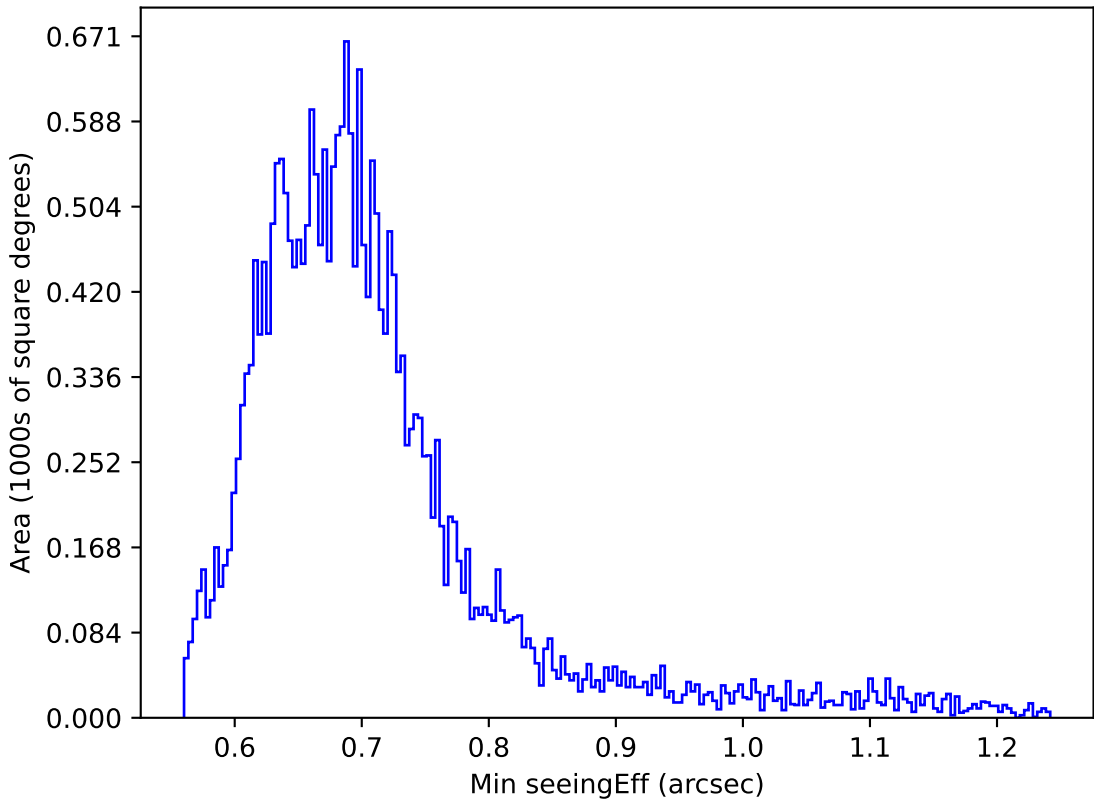
too_elab_r256_d2_ugrizy_v3.4_10yrs Yr 1 r band: Min seeingEff
