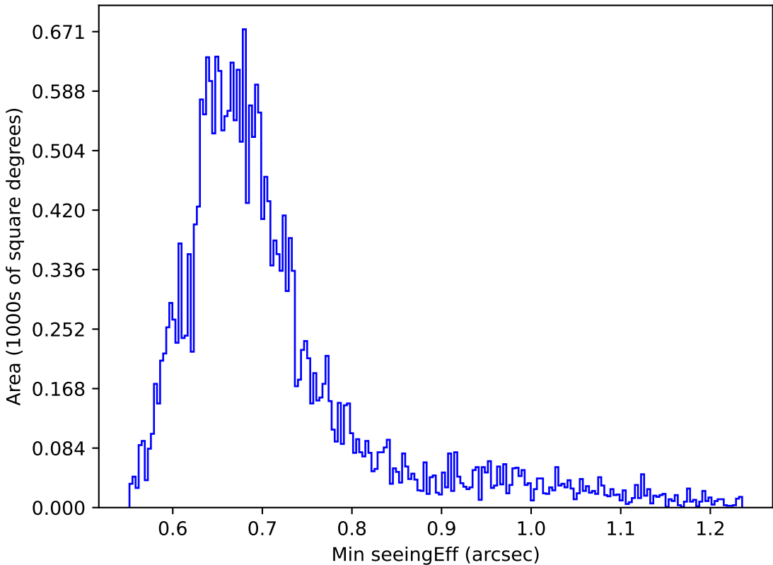
too_elab_r256_d2_ugrizy_v3.4_10yrs Yr 1 i band: Min seeingEff
