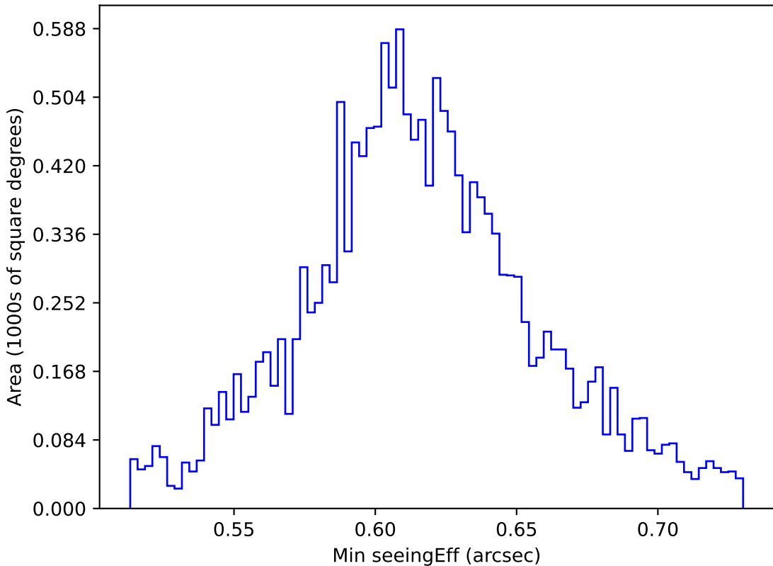
too_elab_r256_d2_ugrizy_v3.4_10yrs WFD z band: Min seeingEff
