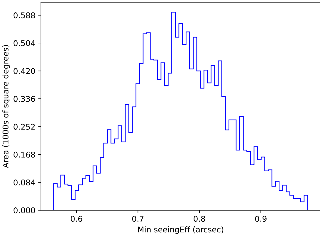
too_elab_r256_d2_ugrizy_v3.4_10yrs WFD u band: Min seeingEff
