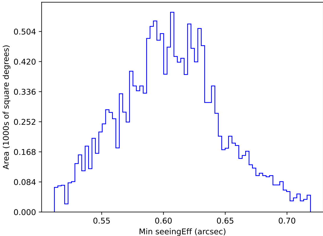
too_elab_r256_d2_ugrizy_v3.4_10yrs WFD i band: Min seeingEff
