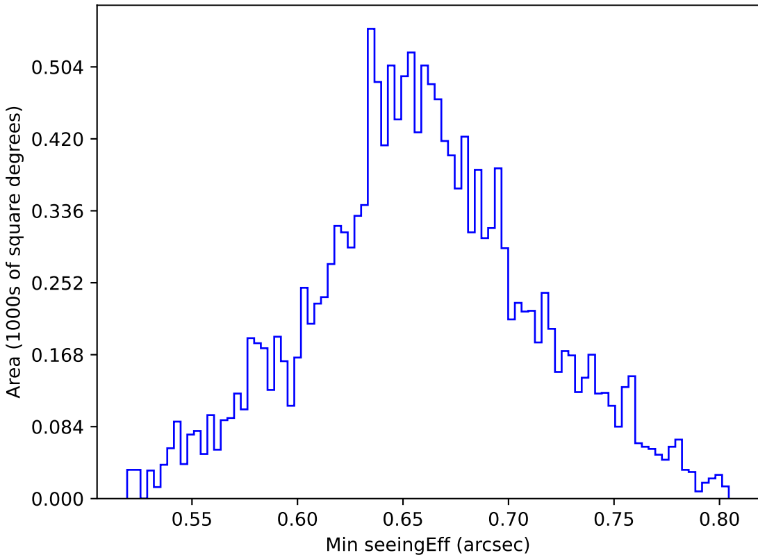
too_elab_r256_d2_ugrizy_v3.4_10yrs WFD g band: Min seeingEff
