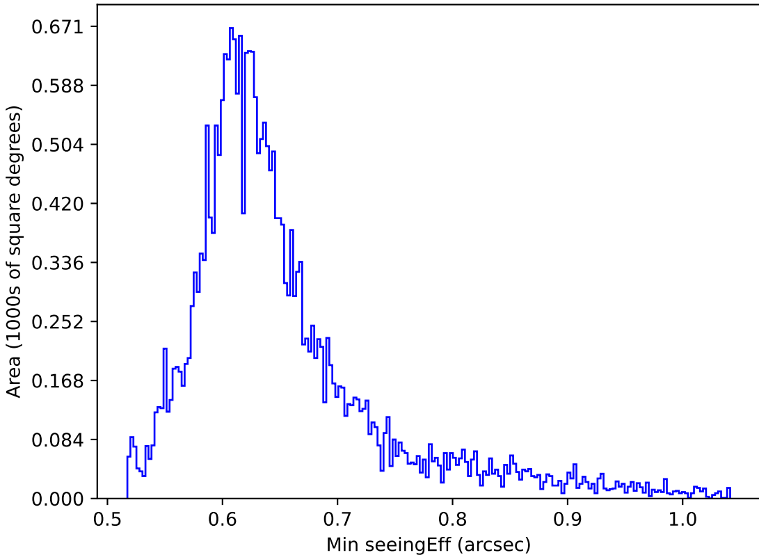
too_elab_r256_d2_ugrizy_v3.4_10yrs All sky z band: Min seeingEff
