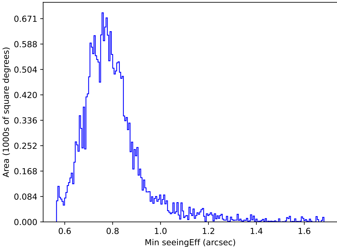
too_elab_r256_d2_ugrizy_v3.4_10yrs All sky u band: Min seeingEff
