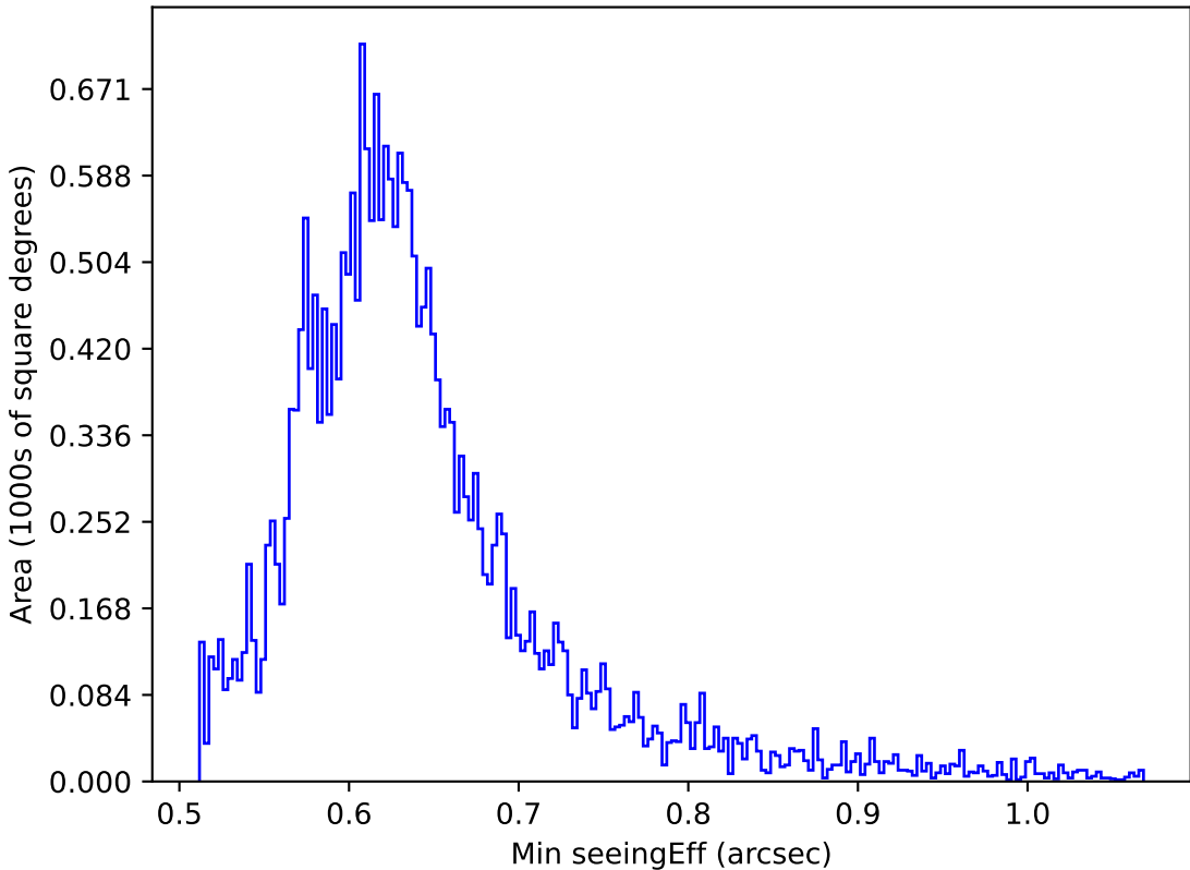
too_elab_r256_d2_ugrizy_v3.4_10yrs All sky r band: Min seeingEff
