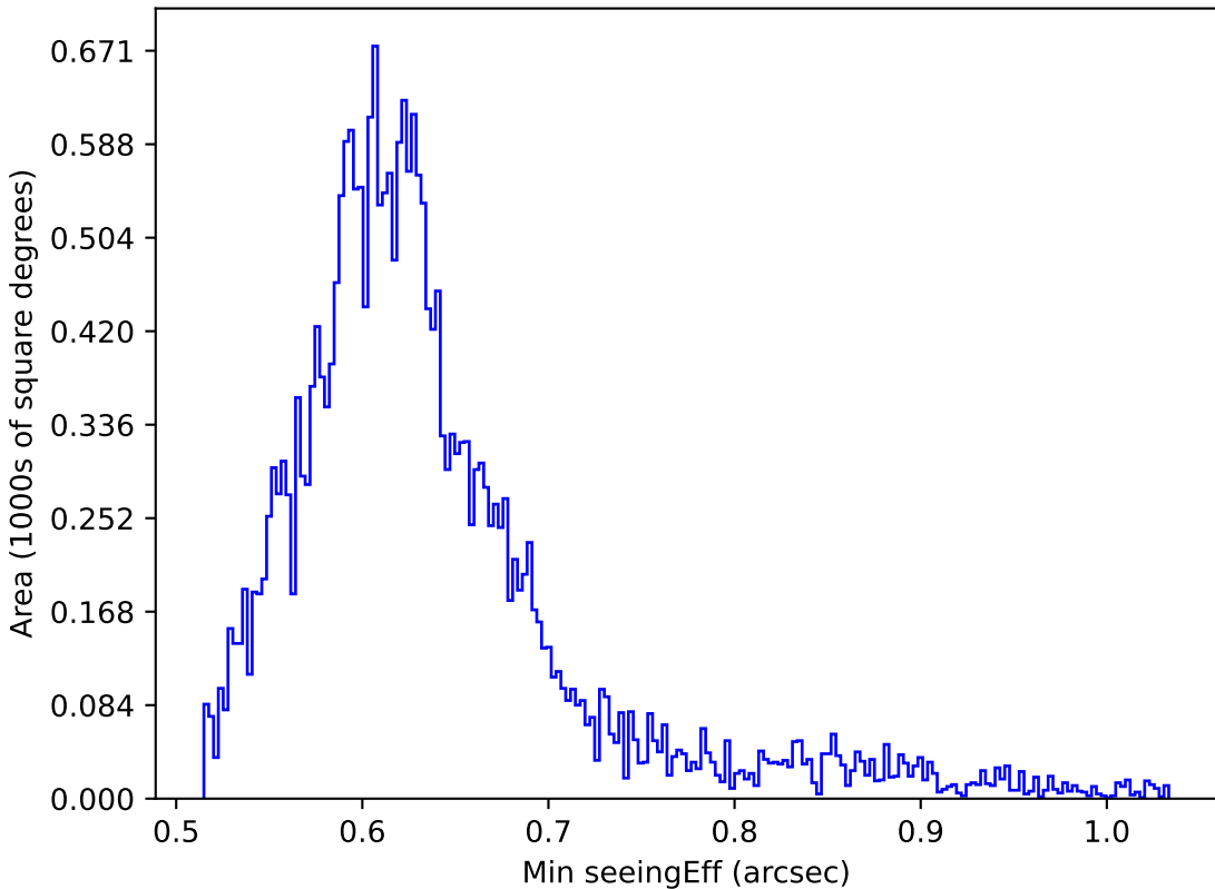
too_elab_r256_d2_ugrizy_v3.4_10yrs All sky i band: Min seeingEff
