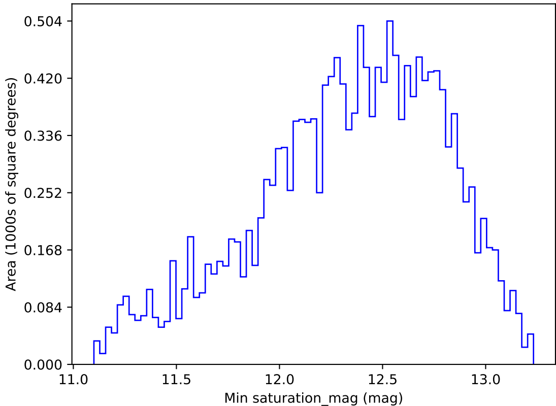
too_elab_r256_d2_ugrizy_v3.4_10yrs WFD i band: Min saturation_mag
